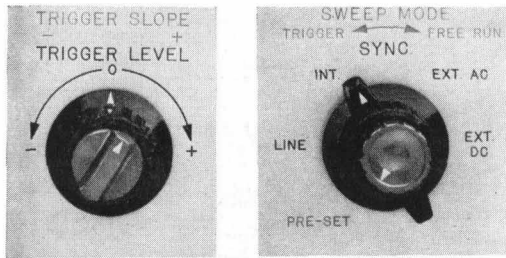
Fig. 5. Trigger controls on new hp-Model 130A . Concentric level- and slope-selecting controls are at left. Sync control at right selects source of trigger voltage. Sweep Mode adjusts sweep for free-running or triggered operation with Preset automatic triggering position at ccw end.
