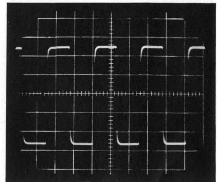
Fig. 9. Oscillogram of 40 kc square wave applied to vertical system. Sweep speed is 10 μsec/cm.
